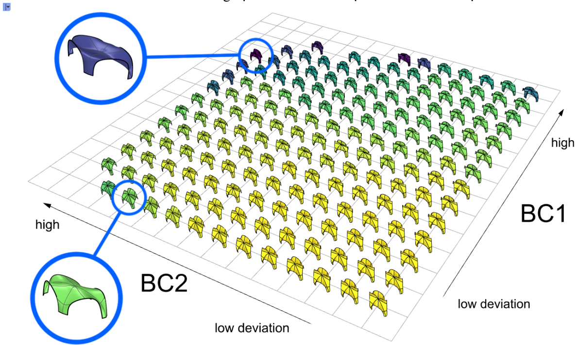
Figure 6: Visualisation of all feasible solutions found in a single run of the FI-MAP-Elites algorithm on the Complex Test Case. Meshes in yellow have a higher fitness (i.e. lower elastic energy)
