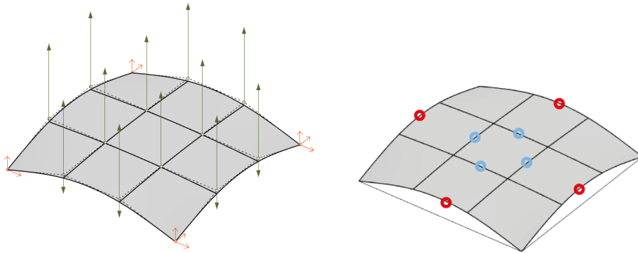
Figure 3: The square base test case, with the height variability range (left), and the BCs calculated based on the average height of the centre points (blue dots in right image) and height difference between arches (red dots in right image).
